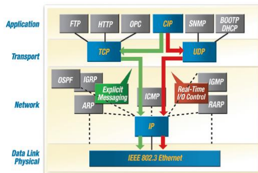
Figura 85 – Arquitetura Explicit e Implicit Messaging “EtherNet/IP™ Quick Start for Vendors Handbook (PUB213R0) ODVA”
